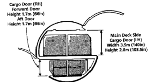
Cross Section Boeing MD-11F
